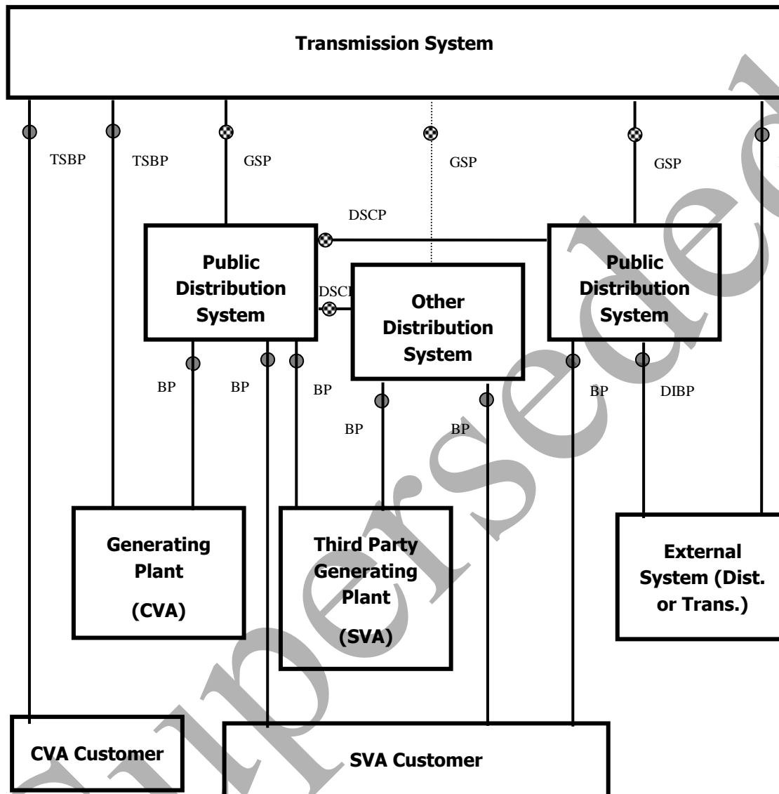
. FIGURE 1 IMPORT AND EXPORT ACTIVE ENERGY FLOWS CONVENTION
