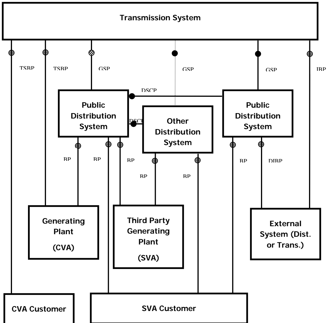
IMPORT AND EXPORT ACTIVE ENERGY FLOWS CONVENTION
